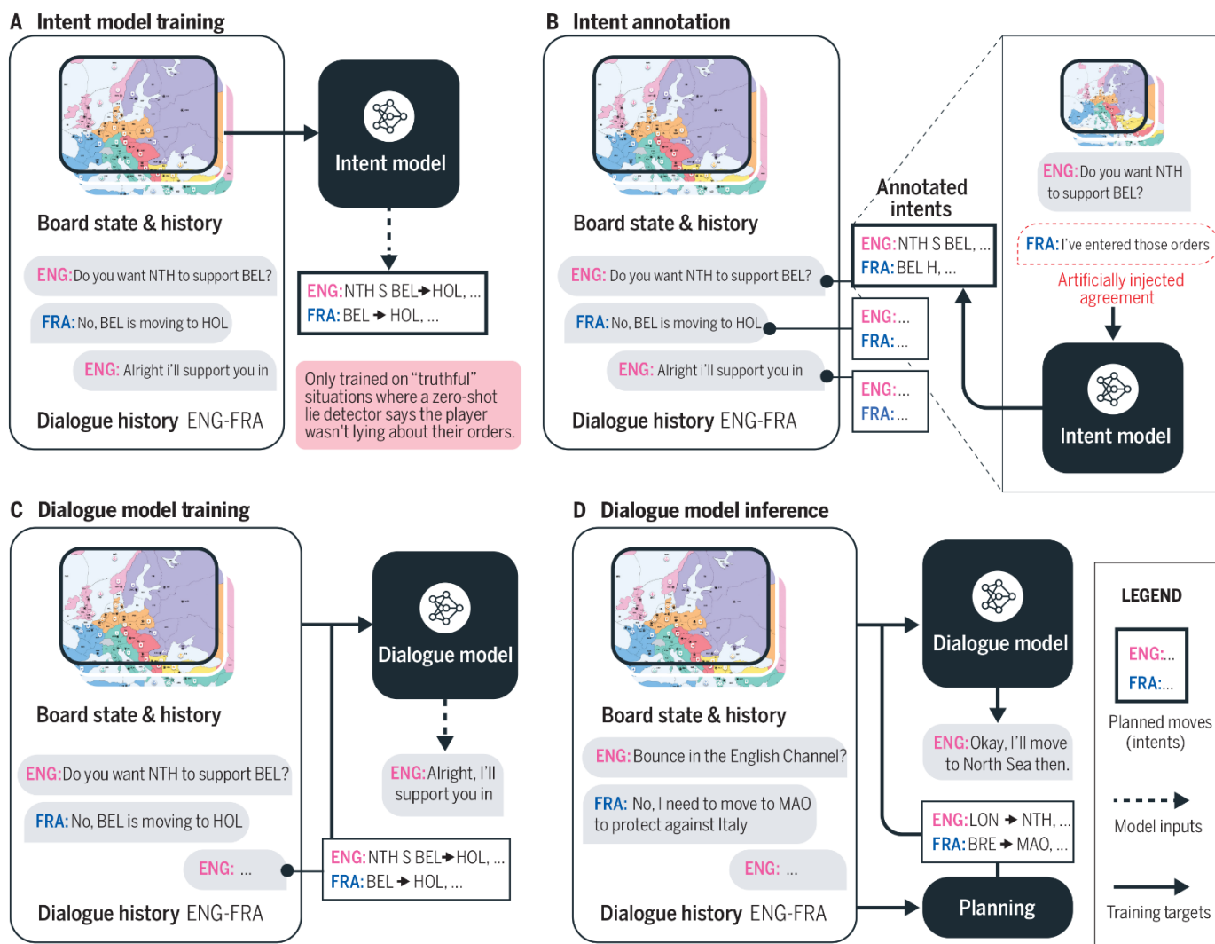
Fig. 2. Illustration of the training and inference process for intent-controlled dialogue. Actions are specified as strings of orders for units, e.g., "NTH S BEL - HOL" means that North Sea will support Belgium to Holland. (A) An 'intent model' was trained to predict actions for a pair of players based on their dialogue. Training data was restricted to a subset where dialogue is deemed 'truthful' (see sup:latent_intents). (B) Each message in the dialogue training dataset was annotated with the output of the intent model on the dialogue up to that point, with an agreement message injected at the end. (C) The dialogue model was trained to predict each dataset message given the annotated intent for the target message. (D) During play, intents were supplied by the planning module instead.
