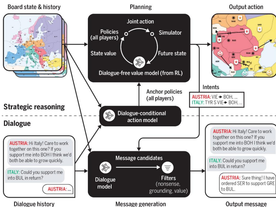
Fig. 1. Architecture of Cicero. Cicero predicts likely human actions for each player based on the board state and dialogue, using that as the starting point for a planning algorithm using RL-trained models. The output of planning is an action for the agent as well as beliefs about other players' actions, which are used to select intents for a dialogue model to condition on. Generated message candidates undergo several filtering steps before a final message is sent.
